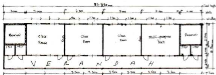
FLOOR PLAN SCALE 1:100
