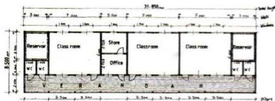
FLOOR PLAN SCALE 1:100
